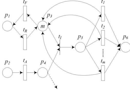
Figure 1. Cluster model.
