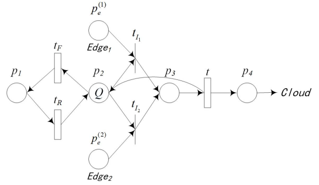
Figure 2. Communication model.
